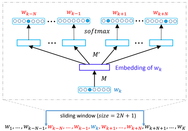
Figure 2: The continuous skip-gram model.
